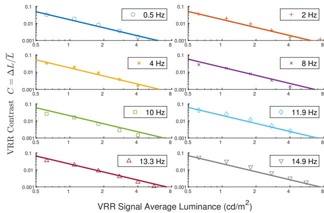
Fig. 3. The contrast of VRR flicker at varying stimulus luminance and temporal frequencies or refresh rate switch, F_{TRS} [Hz]. Luminance levels above 8 \text{cd/m}^2 are irrelevant to us because none of our VRR experimental data reaches above that luminance.
